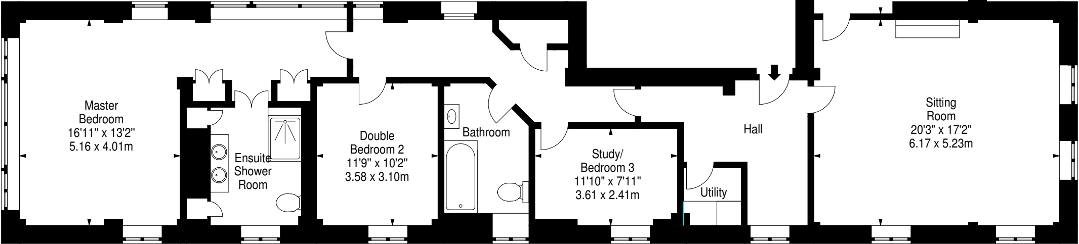
First Floor
