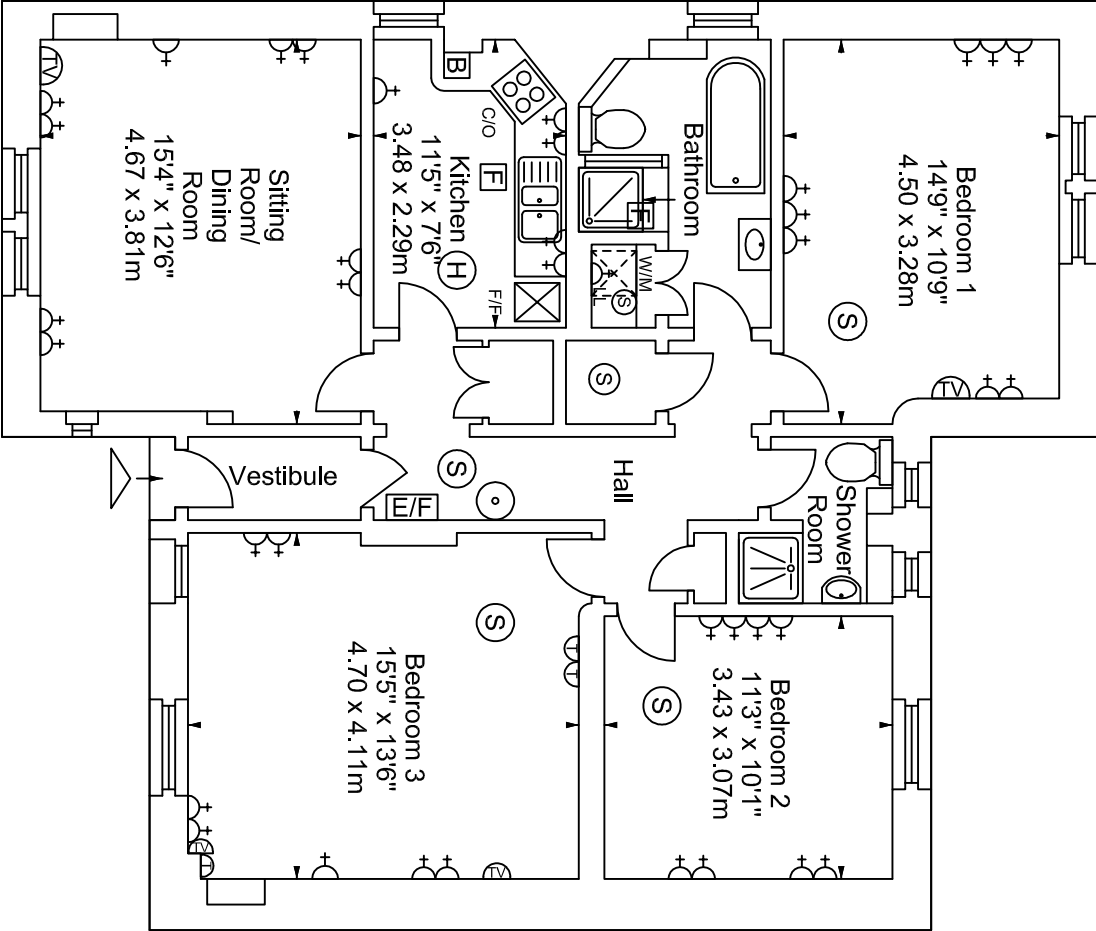
Third Floor
