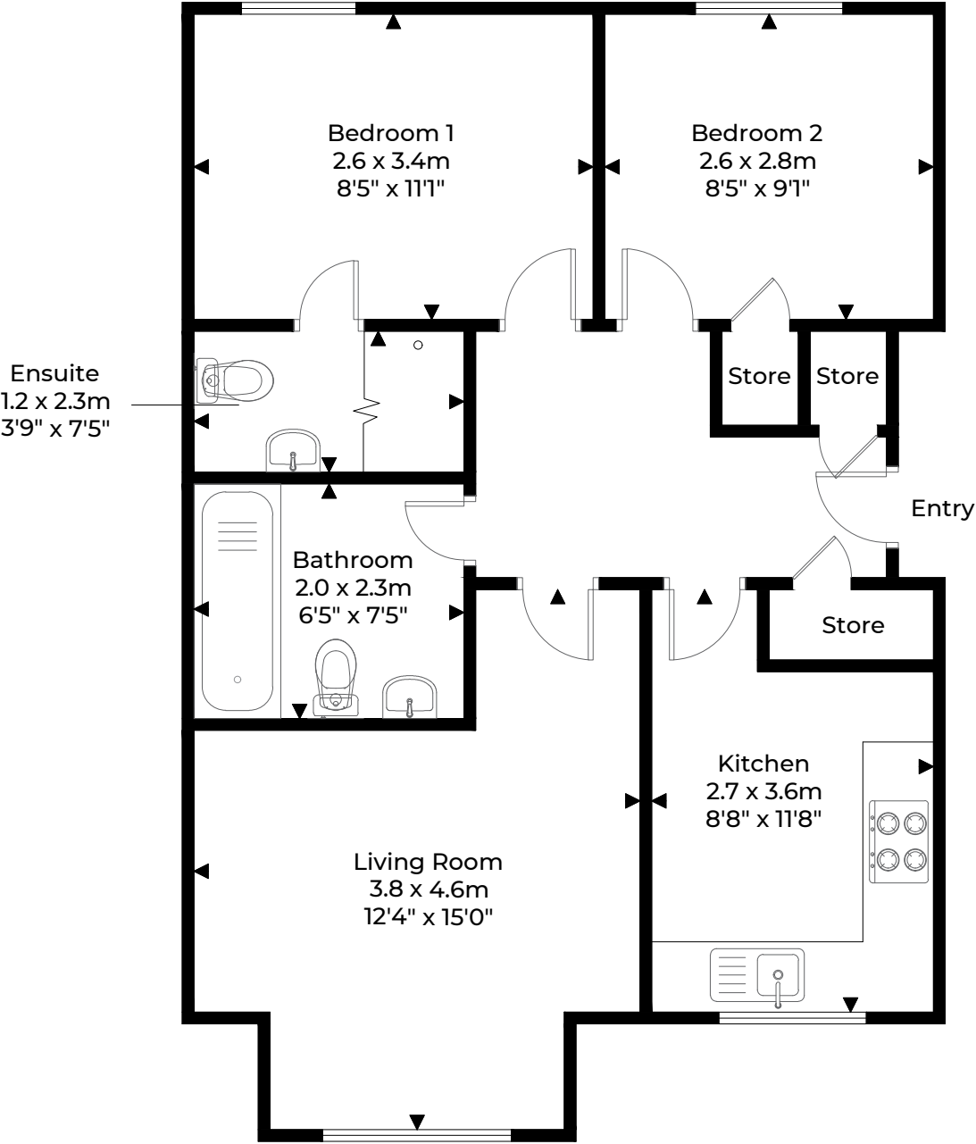
1 st Floor
