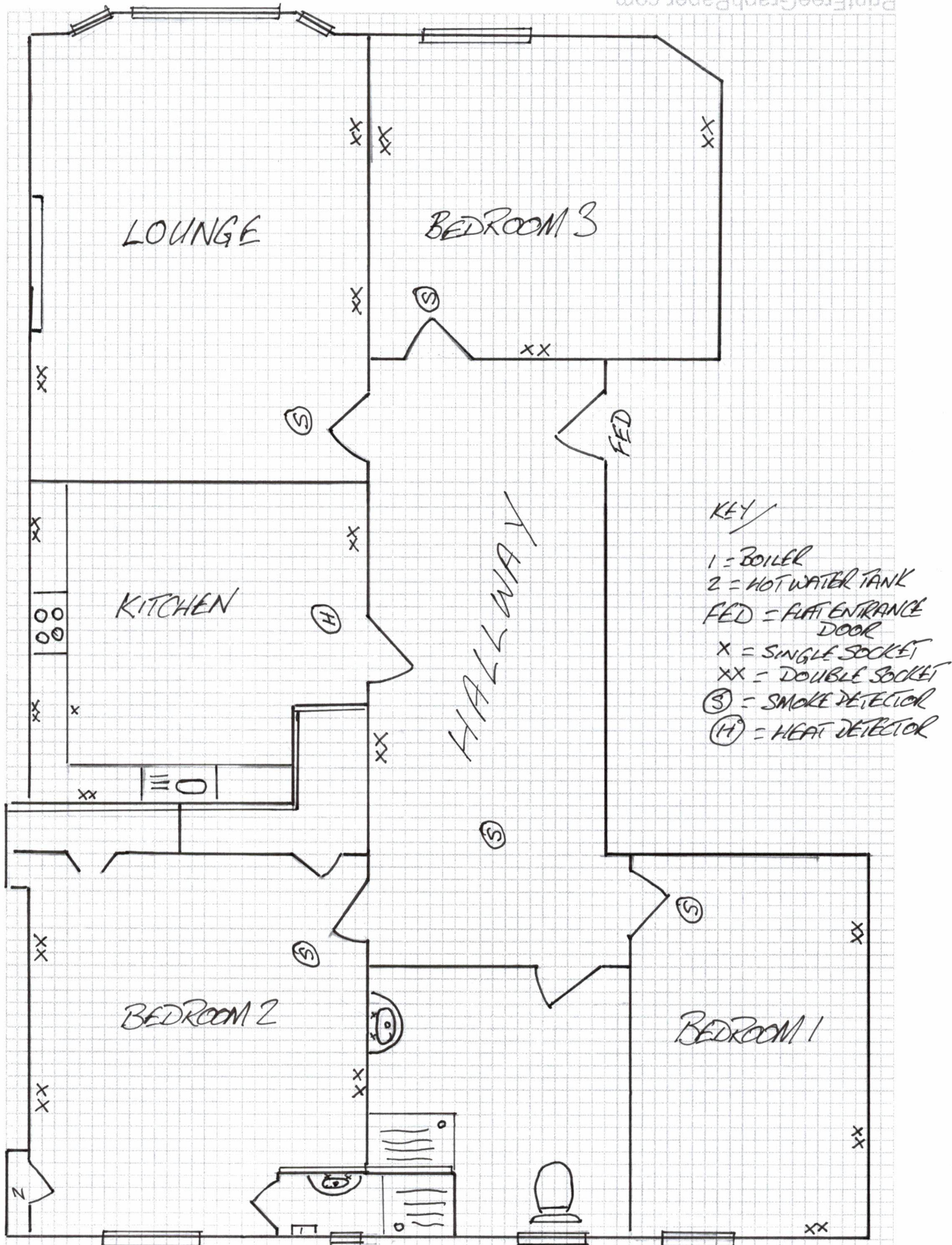
FLOOR PLAN 53 (1F2) BELFORD ROAD NOT TO SCALE
