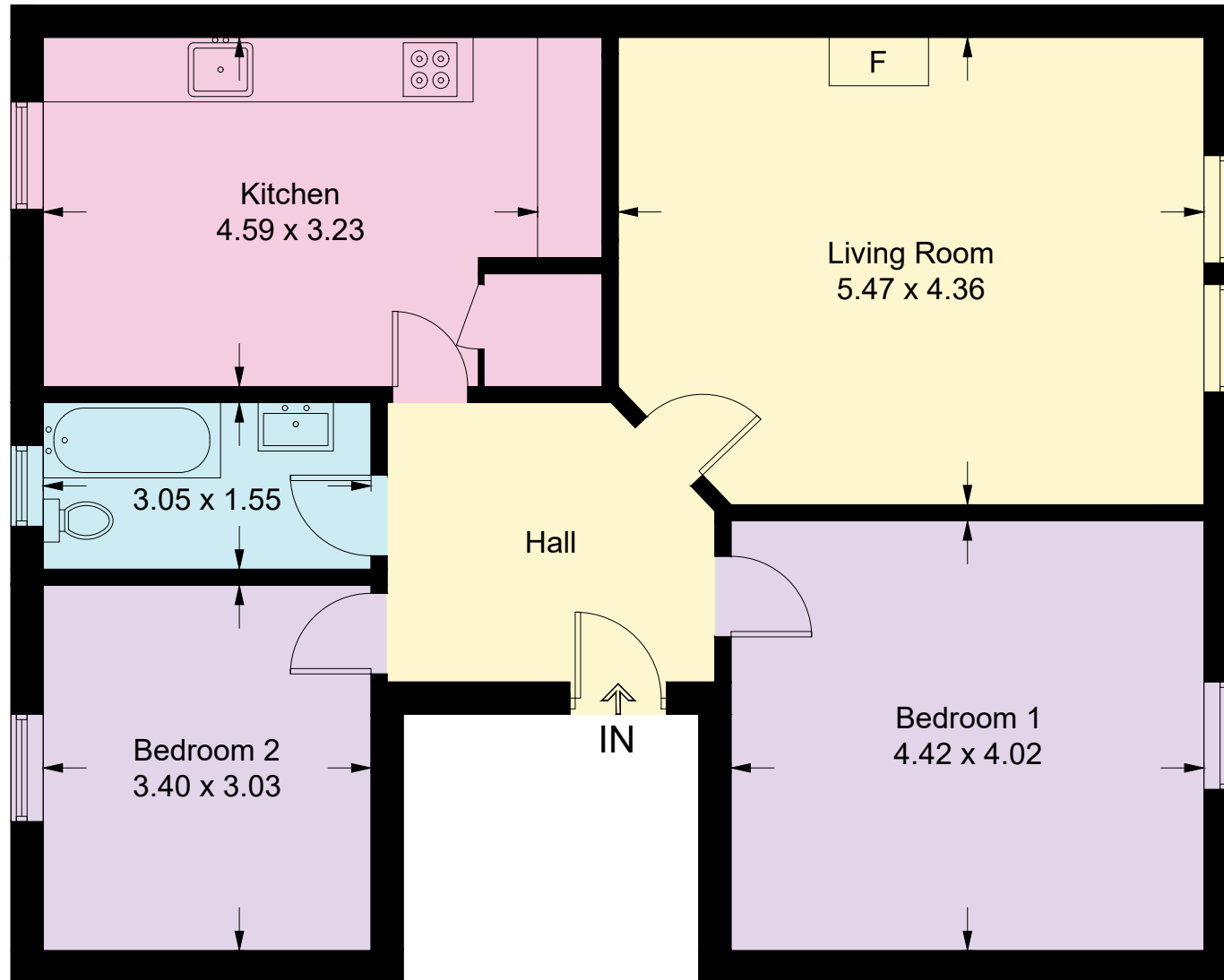
First Floor
