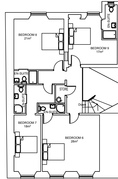
YORK PLACE FIRST FLOOR PLAN
